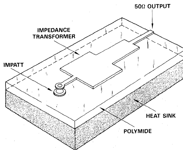
Figure 2 Schematic drawing of monolithic IMPATT oscillator with distributed element impedance matching circuits
