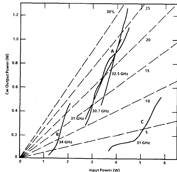
Figure 5 Output powers and efficiencies of Ka-band devices A: Hybrid-Read structure, B: Double-drift, flat-profile, C: Single-drift, flat-profile structure
